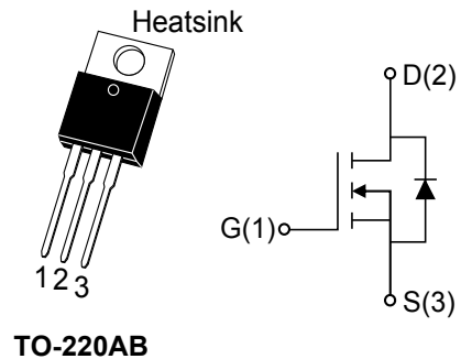
TO-220AB
