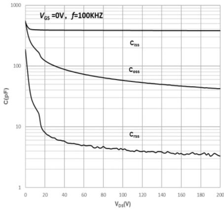
Fig7. Capacitances vs. Drain-Source Voltage (0-200V)
