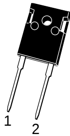
Package:TO-247AC-A ZFP7512A ZFP7512A-HF HF=Halogen Free
