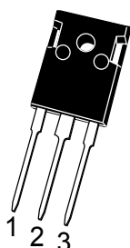
Package:TO-247AB EBR30LH200PT EBR30LH200PT-HF HF=Halogen Free
