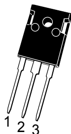
Package:TO-247AB MBR40LH200PT MBR40LH200PT-HF HF=Halogen Free
