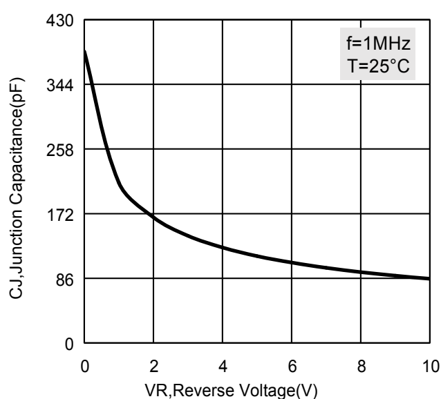
Fig4. Typical Junction Capacitance and Reverse Voltage
