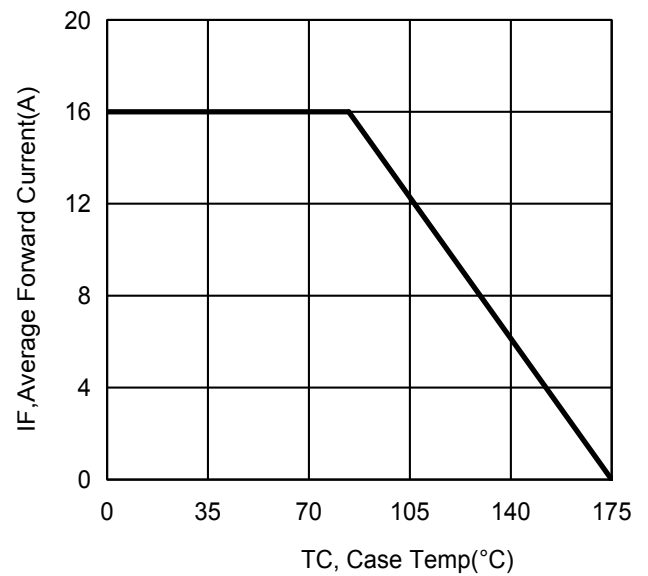
Fig2. Typical Current Derating Curve, Prrlement
