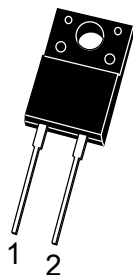
Package: ITO-220AC SFF1265A SFF1265A-HF HF=Halogen Free
