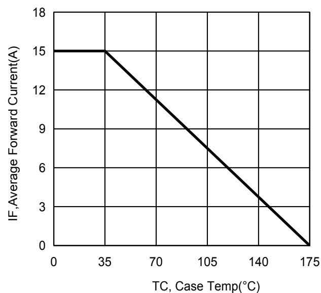
Fig2. Typical Current Derating Curve, Prrlement
