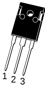
Package:TO-247AB SFP3006AT SFP3006AT-HF HF=Halogen Free
