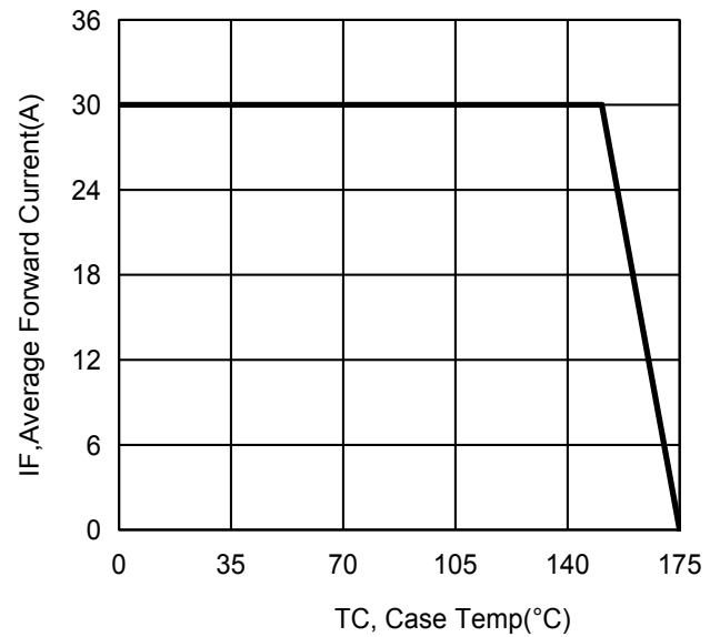
Fig2. Typical Current Derating Curve, Porelement
