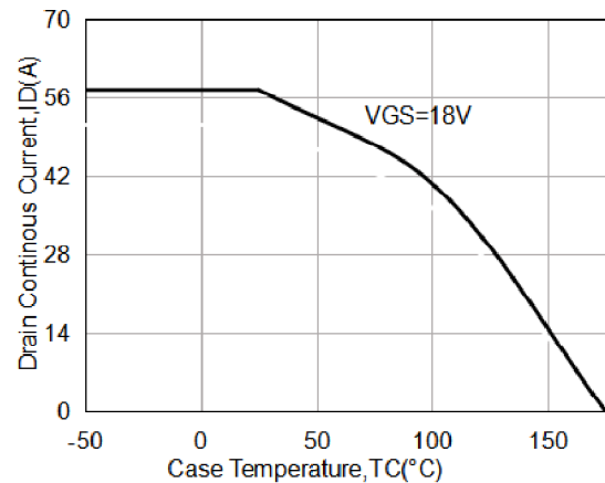
Fig12. Continuous Drain Current Derating vs. Case Temperature
