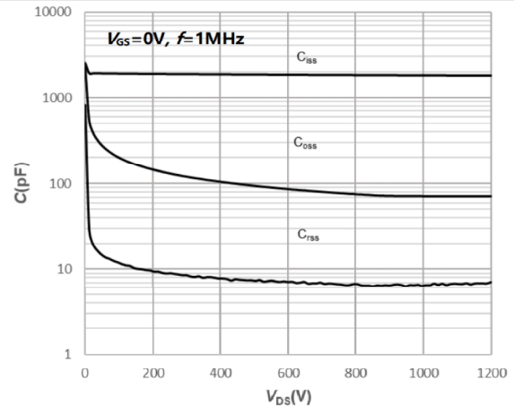
Fig10. Capacitances vs. Drain-Source Voltage(0-1200V)
