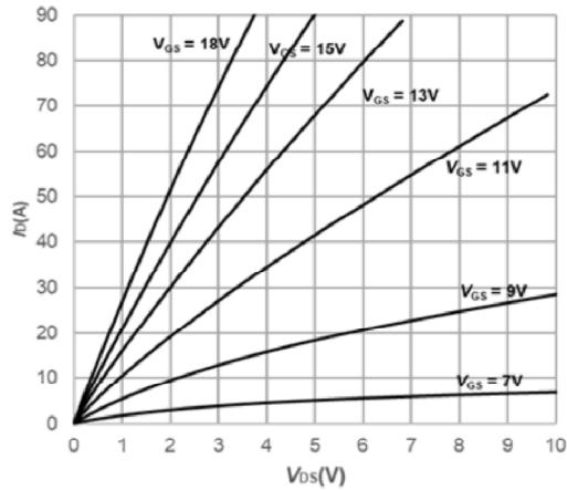
Fig1. Output Characteristics T_j = -55^\circ\text{C}
