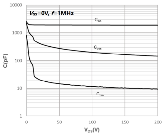
Fig9. Capacitances vs. Drain-Source Voltage(0-200V)
