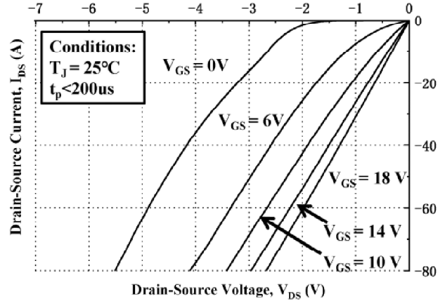
Fig14. 3rd Quadrant Characteristic at T_J = 25^\circ\text{C}
