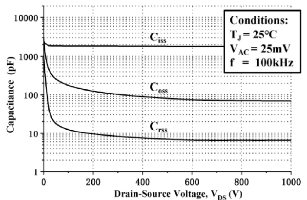
Fig18. Capacitances vs. Drain-Source Voltage(0-1000V)
