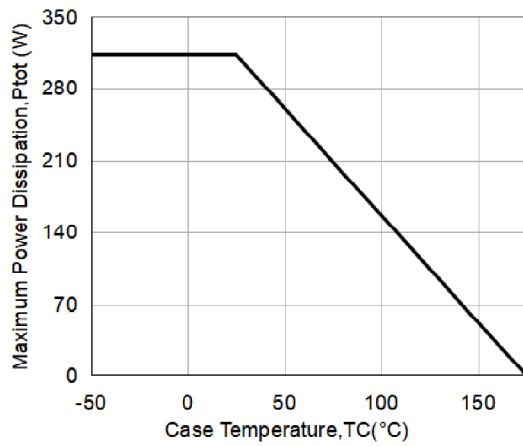
Fig19. Maximum Power Dissipation Derating vs. Case Temperature
