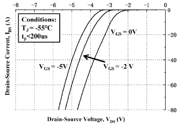
Fig8. Body Diode Characteristic at T_J = -55^\circ C
