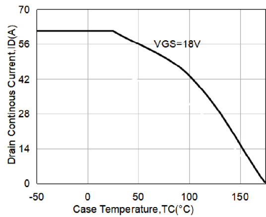
Fig20. Continuous Drain Current Derating vs. Case Temperature
