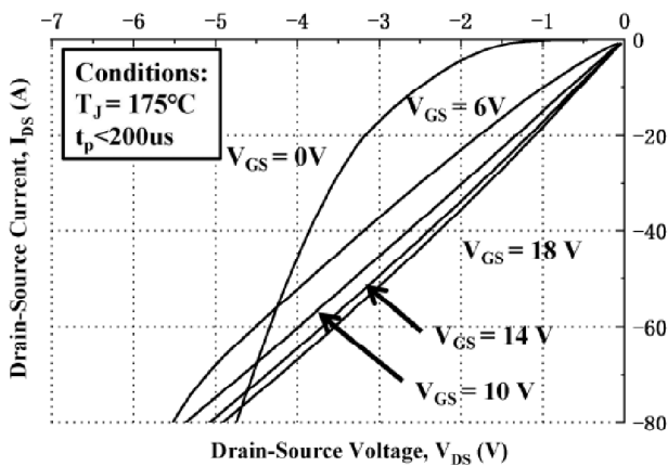
Fig15. 3rd Quadrant Characteristic at T_J = 175^\circ\text{C}
