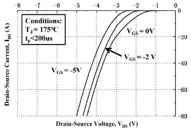
Fig10. Body Diode Characteristic at T_J = 175^\circ C
