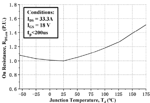
Fig5. Normalized On-Resistance vs. Temperature
