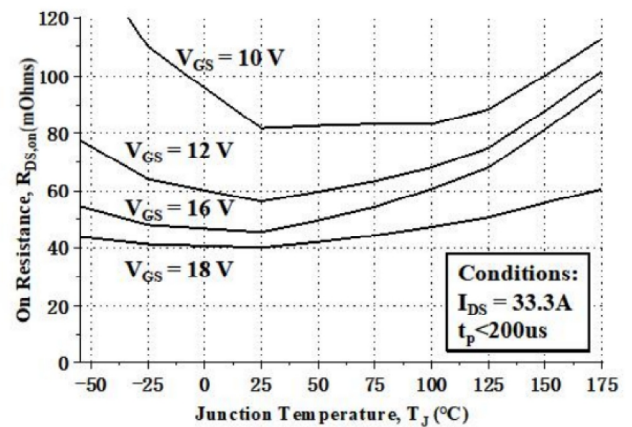
Fig4. On-Resistance vs. Temperature For Various Gate Voltages
