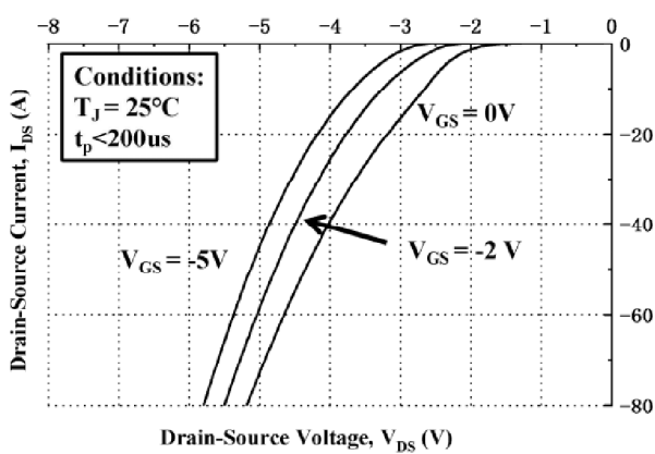
Fig9. Body Diode Characteristic at T_J = 25^\circ C
