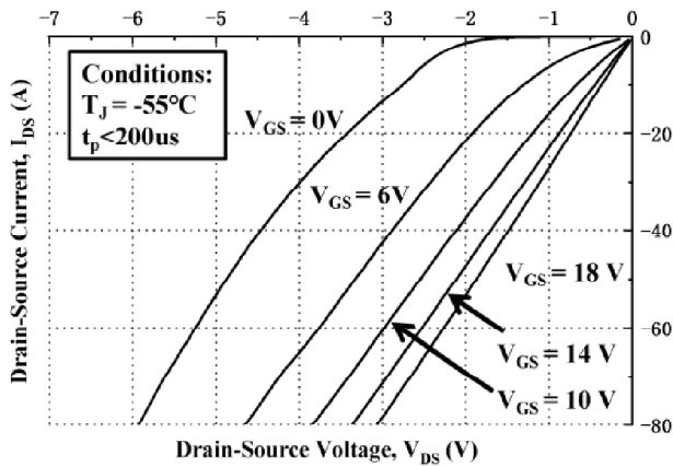
Fig13. 3rd Quadrant Characteristic at T_J = -55^\circ\text{C}
