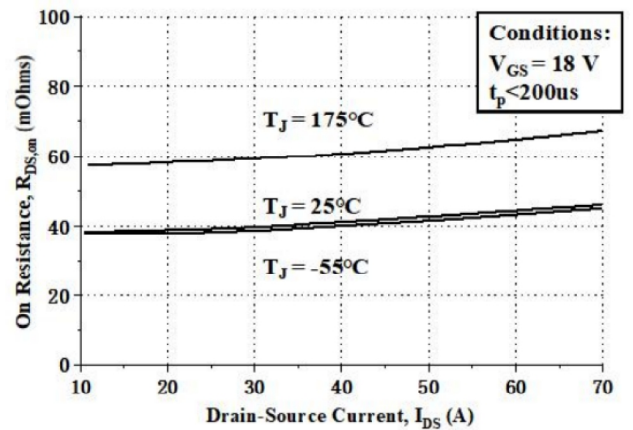
Fig6. On-Resistance vs. Drain Current For Various Temperatures
