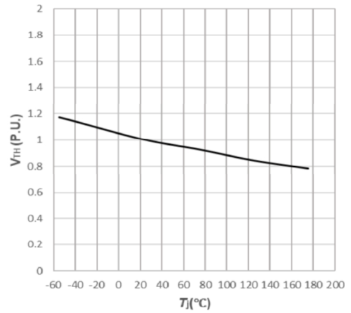
Fig8. Normalized Threshold Voltage vs. Temperature
