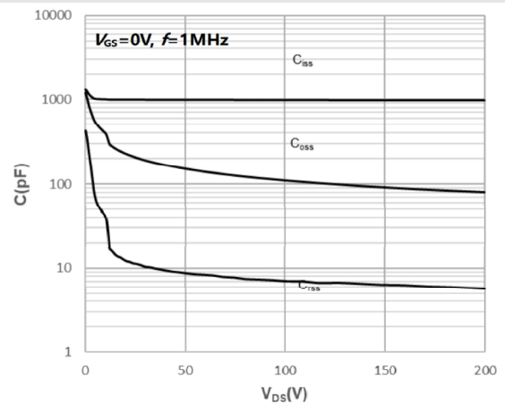
Fig10. Capacitances vs. Drain-Source Voltage(0-200V)
