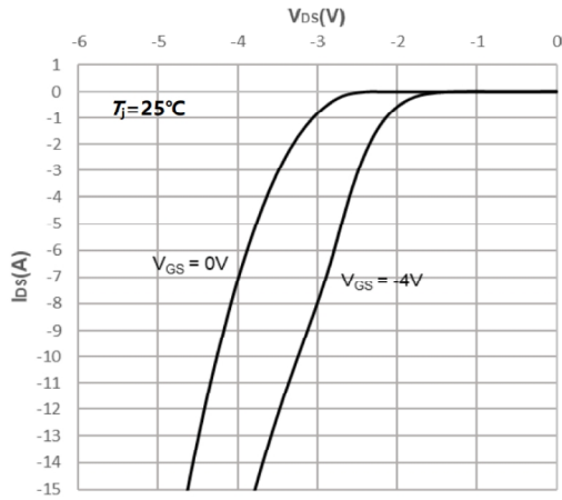
Fig7. Body Diode Characteristic at T_j=25^\circ\text{C}
