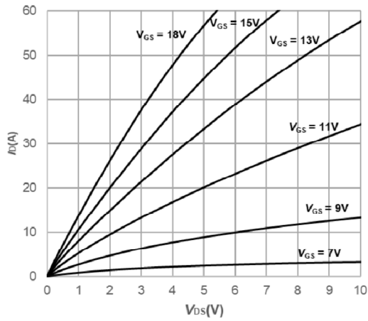
Fig1. Output Characteristics T_j = -55^\circ\text{C}
