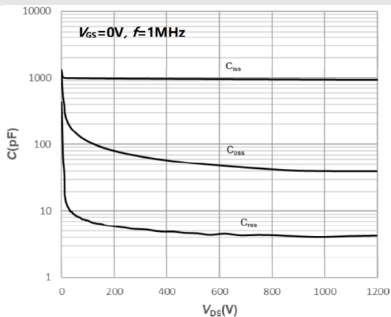
Fig11. Capacitances vs. Drain-Source Voltage(0-1200V)
