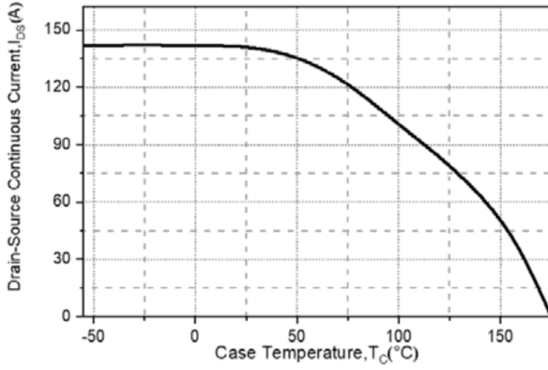
Fig19. Continuous Drain Current vs. Case Temperature
