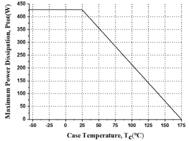
Fig20. Maximum Power Dissipation vs. Case Temperature
