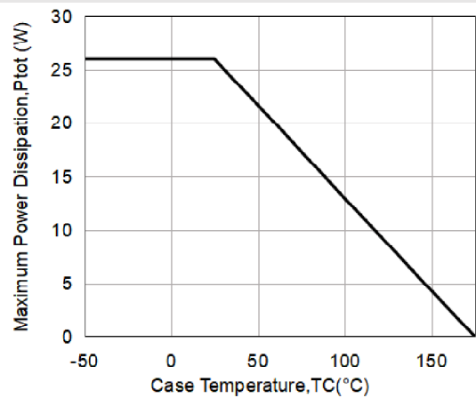
Fig16. Maximum Power Dissipation Derating vs. Case Temperature
