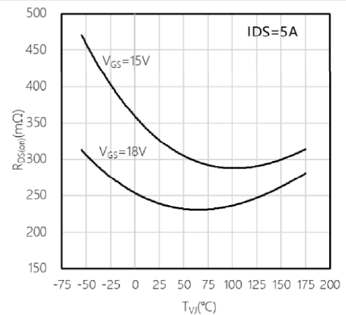
Fig4. On-Resistance vs. Temperature For Various Gate Voltages
