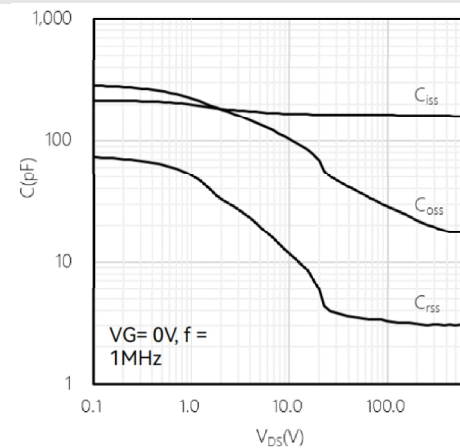
Fig12. Capacitances vs. Drain-Source Voltage(0-200V)
