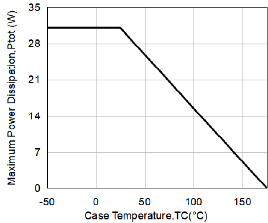
Fig16. Maximum Power Dissipation Derating vs. Case Temperature
