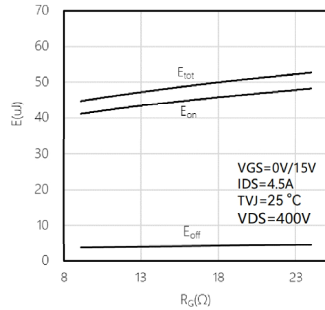
Fig14. Clamped Inductive Switching Energy vs. R_{\text{G}} at T_{\text{J}}=25^\circ\text{C}
