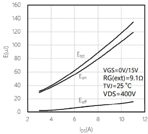
Fig13. Clamped Inductive Switching Energy vs. Drain Current
