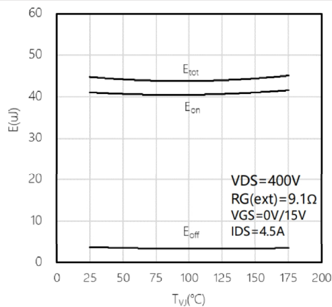
Fig15. Clamped inductive switching energy vs. temperature at T_{\text{J}}=25^\circ\text{C}
