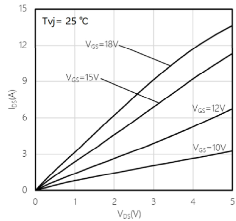
Fig2. Output Characteristics T_j = 25^\circ\text{C}
