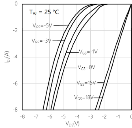
Fig8. Typical Reverse Drain Current vs. Reverse Drain Voltage at Different VGS Tj=25°C
