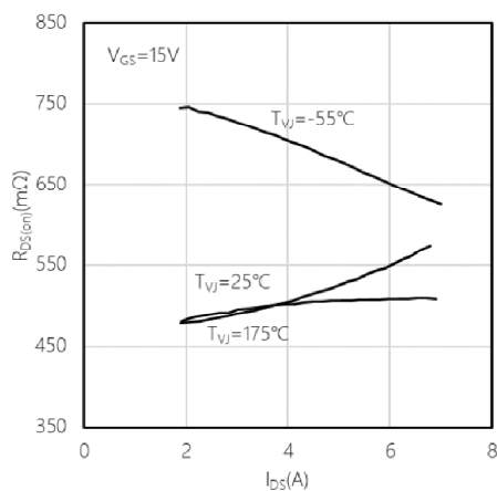
Fig5. On-Resistance vs. Drain Current For Various Temperatures
