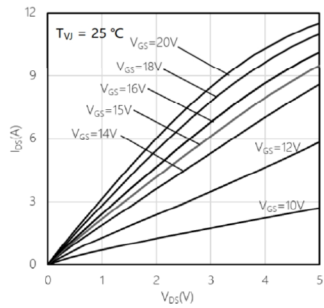
Fig2. Output Characteristics T_j = 25^\circ\text{C}
