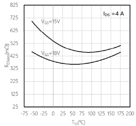
Fig4. On-Resistance vs. Temperature For Various Gate Voltages
