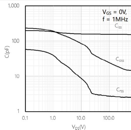
Fig12. Capacitances vs. Drain-Source Voltage(0-200V)
