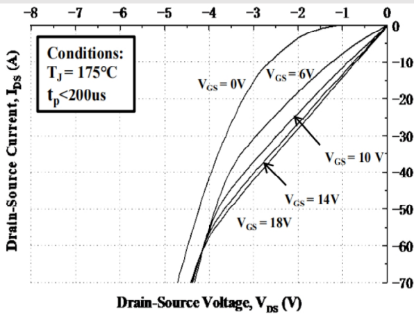
Fig15. 3rd Quadrant Characteristic at 175°C
