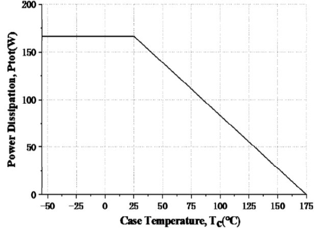
Fig20. Maximum Power Dissipation vs. Case Temperature
