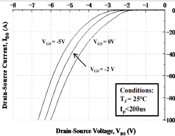
Fig9. Body Diode Characteristic at 25°C
