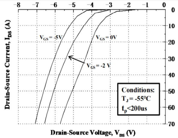
Fig8. Body Diode Characteristic at -55°C
