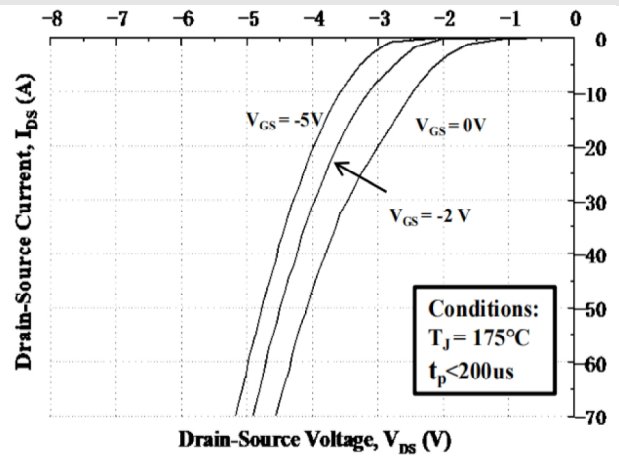
Fig10. Body Diode Characteristic at 175°C
