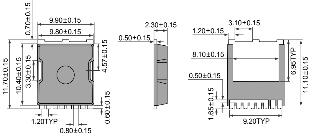
TOLL-8L Unit: mm
