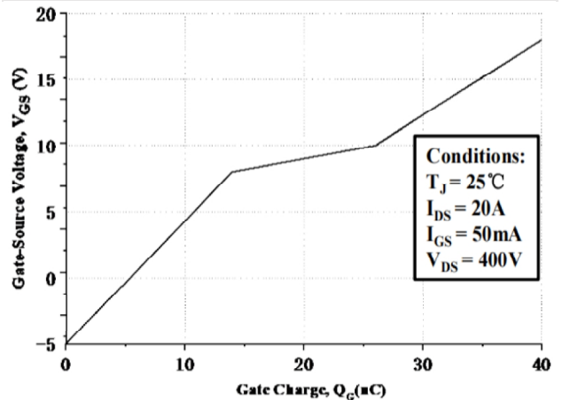
Fig12. Gate Charge Characteristics
