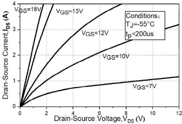
Fig1. Output Characteristics T_J = -55^\circ\text{C}
