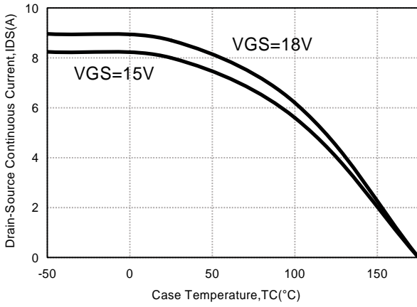
Fig19. Continuous Drain Current vs. Case Temperature
