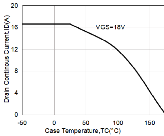
Fig13. Continuous Drain Current Derating vs. Case Temperature
