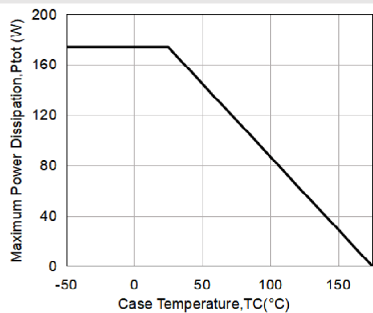
Fig12. Maximum Power Dissipation Derating vs. Case Temperature
