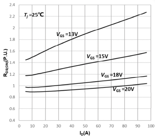
Fig5. Normalized On-Resistance vs. Drain Current For Various Gate Voltages
