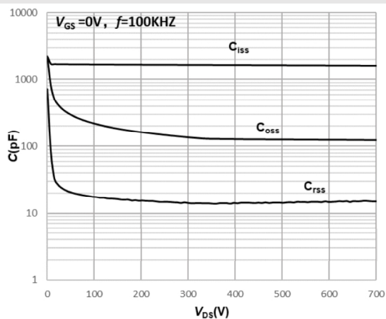
Fig11. Capacitances vs. Drain-Source Voltage(0-700V)
