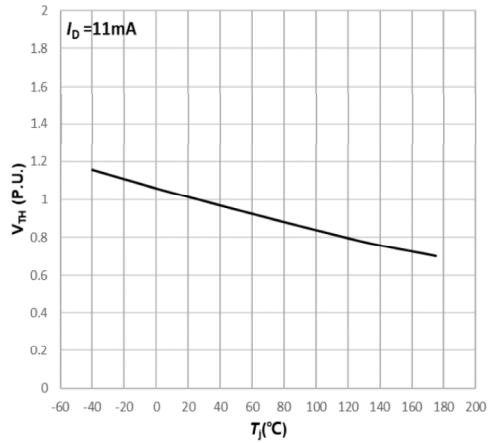
Fig7. Normalized Threshold Voltage vs. Temperature
