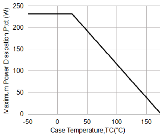
Fig11. Maximum Power Dissipation Derating vs. Case Temperature
