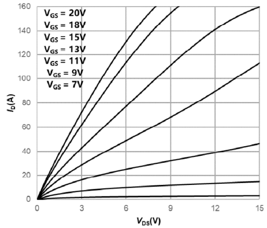
Fig2. Output Characteristics T_j = 25^\circ\text{C}
