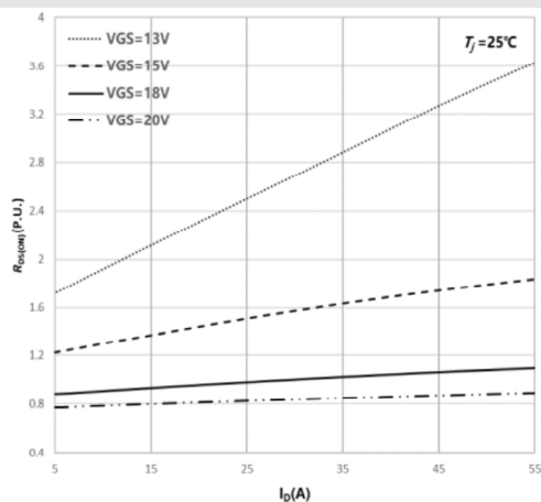
Fig5. Normalized On-Resistance vs. Drain Current For Various Gate Voltages
