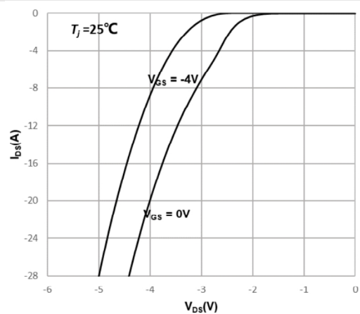
Fig6. Body Diode Characteristic at T_j = 25^\circ\text{C}
