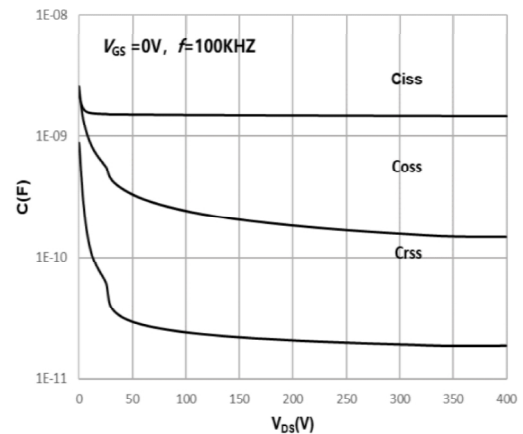
Fig10. Capacitances vs. Drain-Source Voltage(0-400V)
