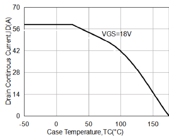
Fig12. Continuous Drain Current Derating vs. Case Temperature
