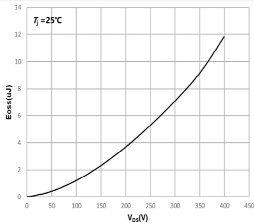
Fig9. Output Capacitor Stored Energy
