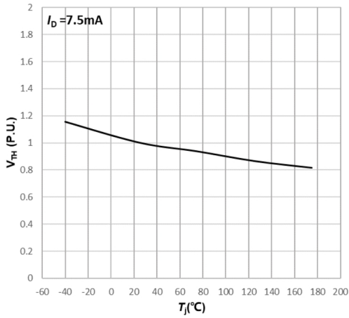
Fig7. Normalized Threshold Voltage vs. Temperature
