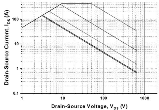
Fig22.Safe Operating Area
