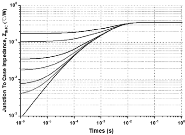
Fig21.Transient Thermal Impedance(Junction-Case)
