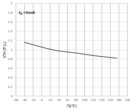
Fig7. Normalized Threshold Voltage vs. Temperature
