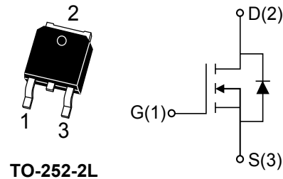
TO-252-2L
