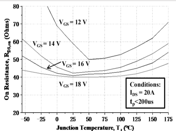
Fig6. On-Resistance vs. Temperature For Various Gate Voltage
