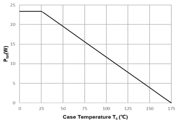
Fig12. Maximum Power Dissipation vs. Case Temperature
