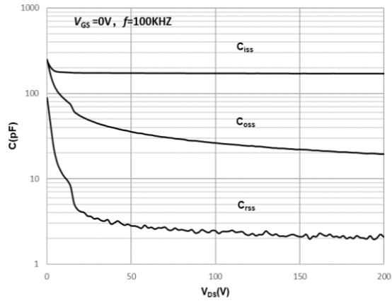
Fig7. Capacitances vs. Drain-Source Voltage (0-200V)
