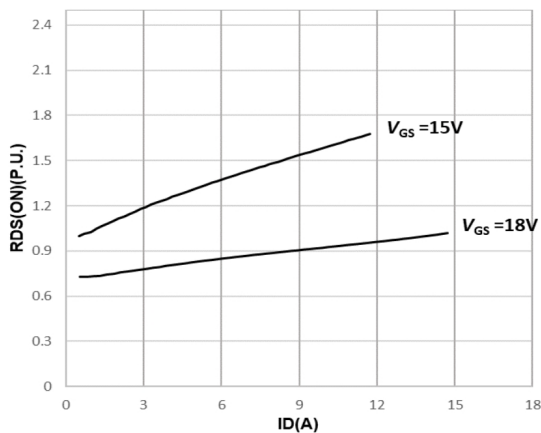
Fig5. Normalized On-Resistance vs. Drain Current For T_j=25^\circ\text{C}
