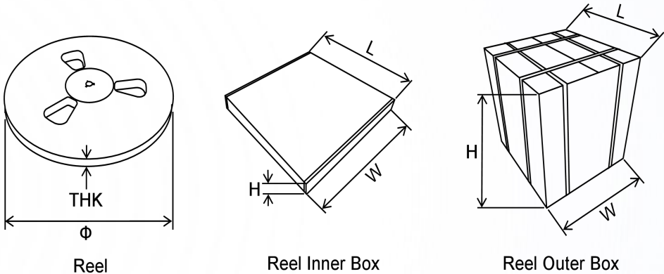
Packaging:Reel
