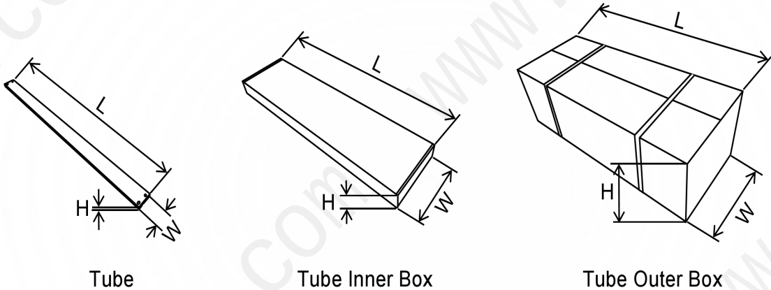
Packaging:Tube
